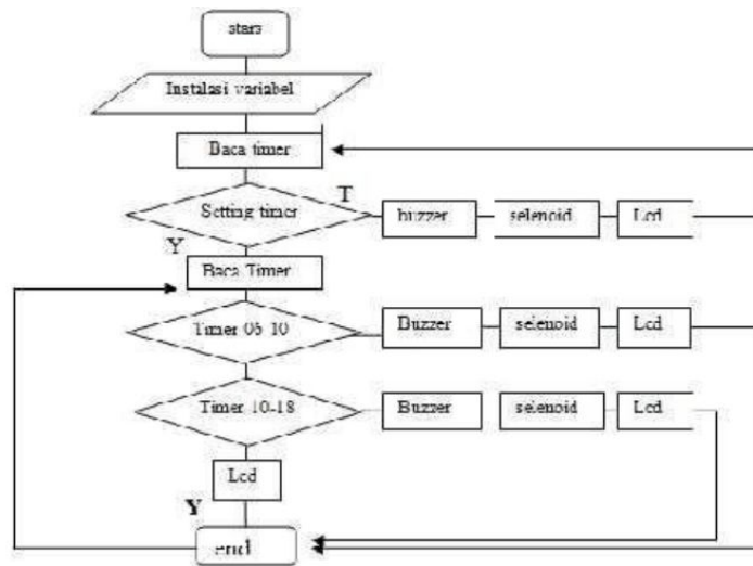
Gambar 4 Rancangan alur diagram Program
