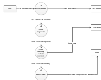
Gambar 6. DFD Level 1.1 Parsing kalimat
