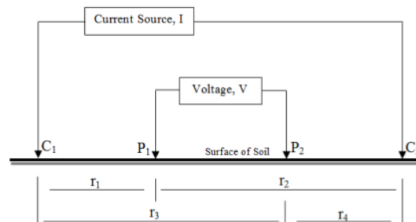
Figure 1. Current electrode and potential electrode [3]
