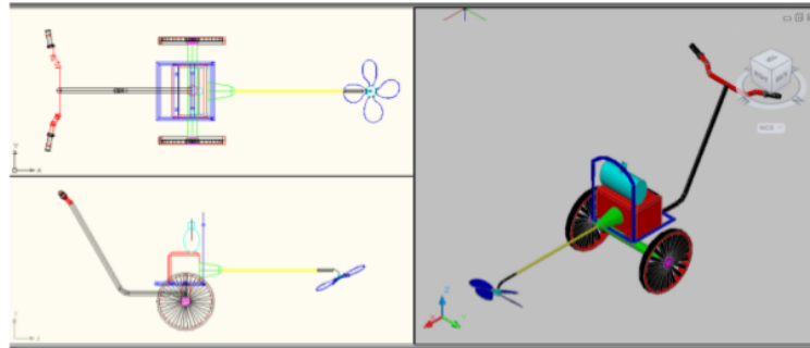
Figure 2. Design of paddy harvesting machine.
