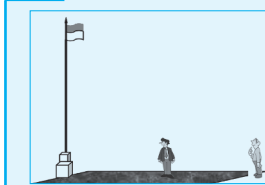
Gambar 8.11 Tiang Bendera
